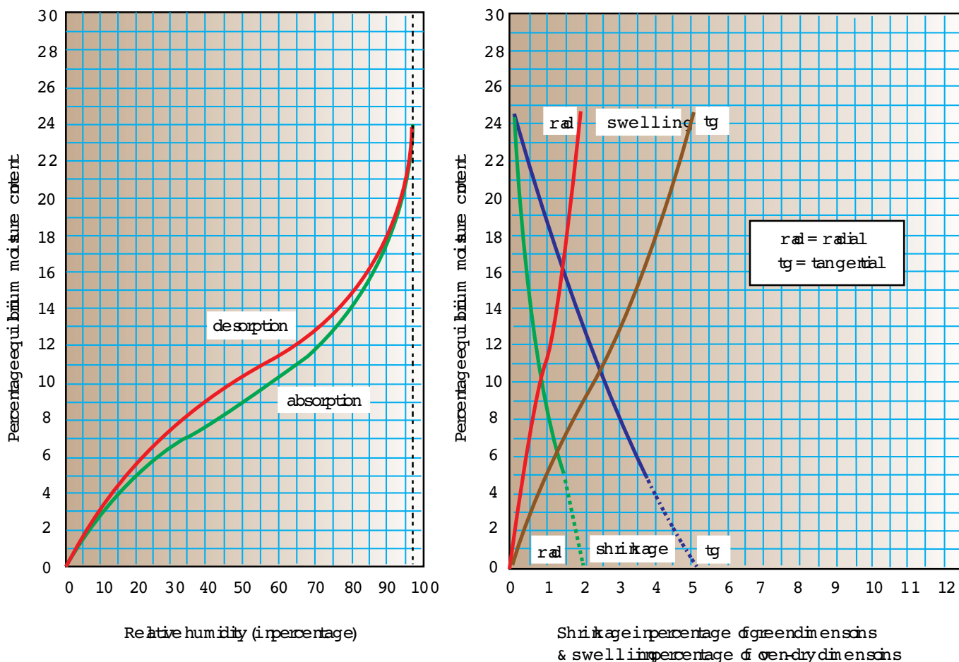
FIGURE 4. Hysteresis, shrinkage and swelling curves of western red cedar (average values of 15 test specimens from 11 trees) (after Rijdsdijk and Laming 1994)
